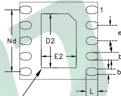
EXPOSED THERMAL PAD ZONE BOTTOM VIEW
